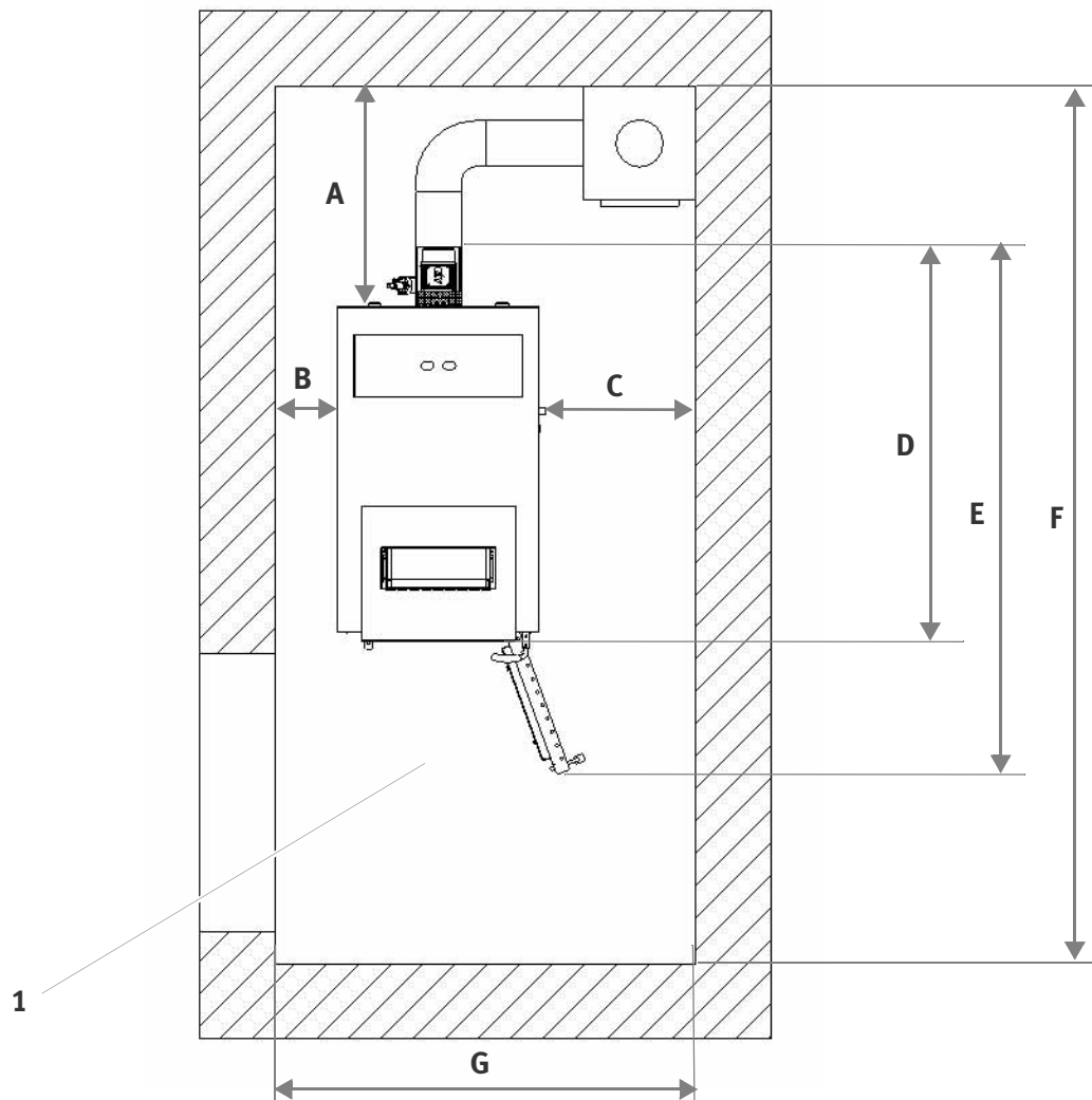
Figure 3/6 - Space and dimensional requirements
